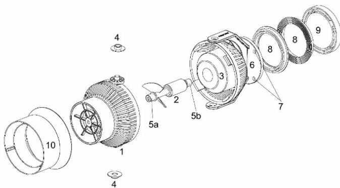
Schéma 1: Construction EcoDrift
