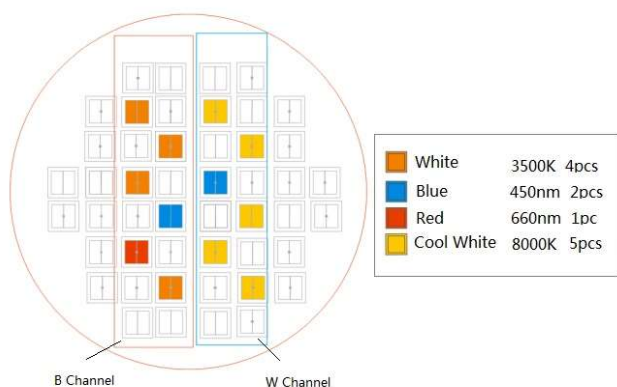
Fig. 2: Qube 30 plant
