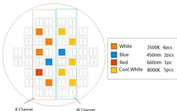
Abb. 2: Qube 30 plant
