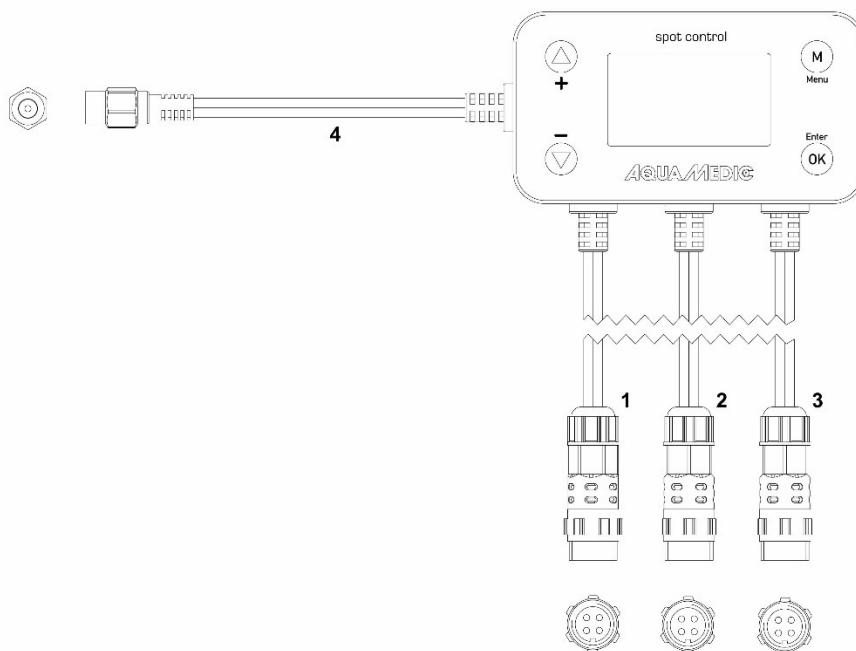
Fig. 1: spot control Connections 1 – 3: control outputs: 1 – 3 Connection 4: power supply unit 12 V
